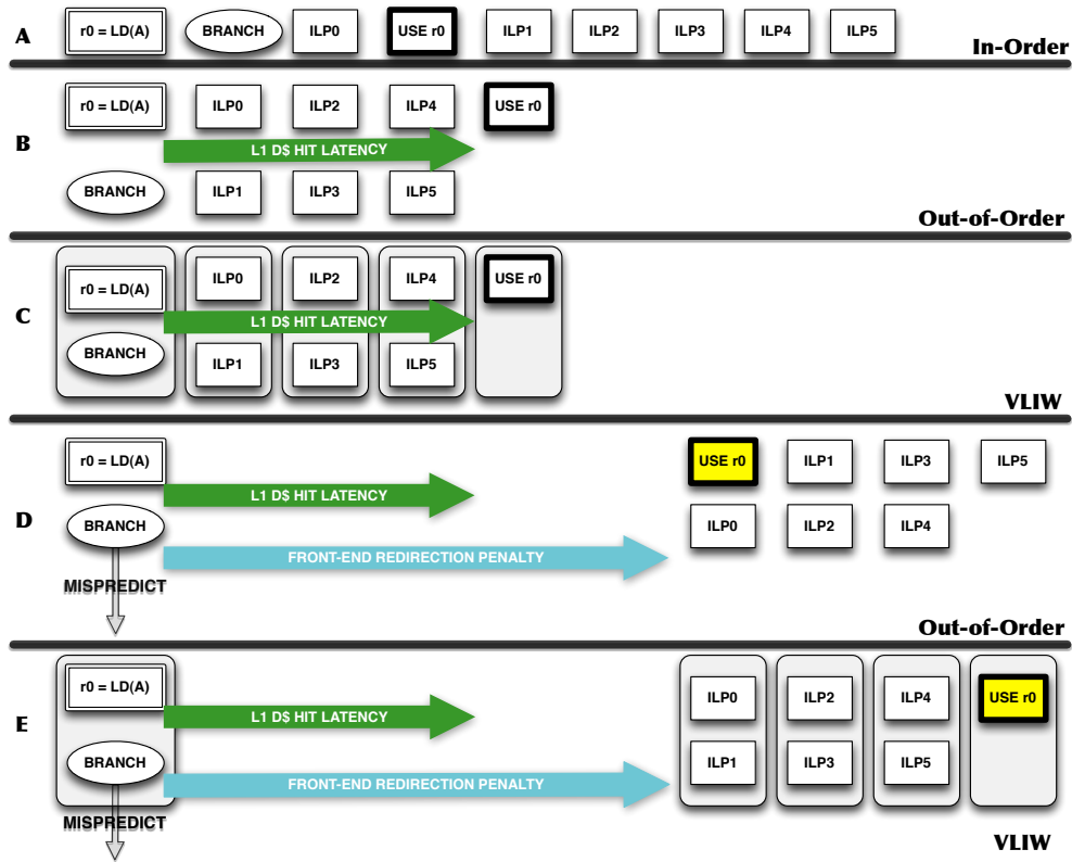
Figure 4. Misprediction recovery latency covers L1-hit latency
