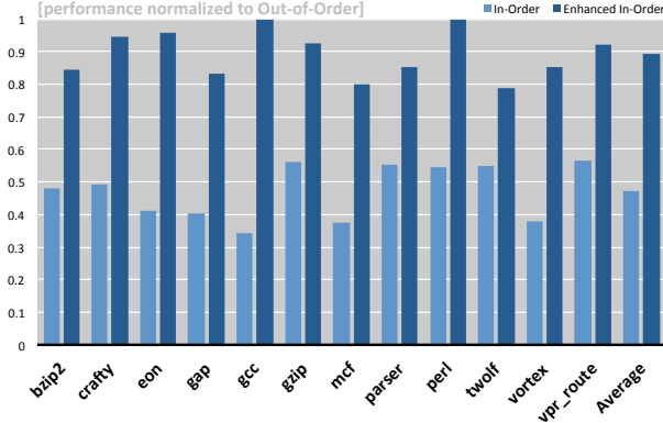
Figure 6. Performance Comparison of the Baseline In-Order and the In-Order Enhanced With Support for Software Speculation
