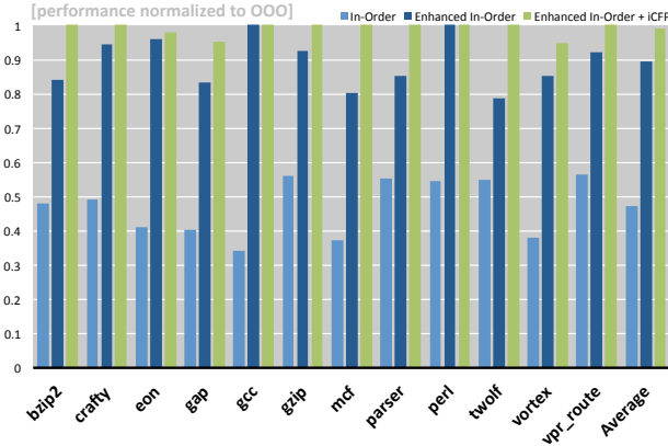
Figure 7. Performance Comparison of the Baseline OOO and the In-Order Enhanced With Support for Software Speculation and iCFP
