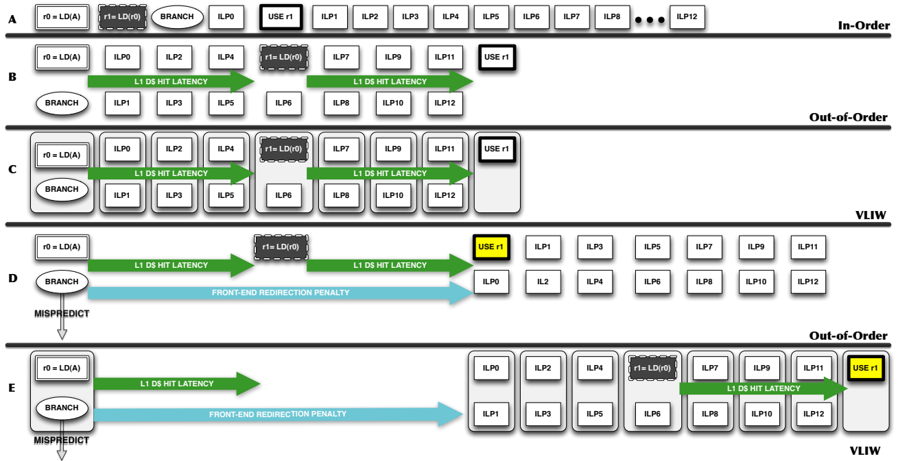
Figure 5. Misprediction recovery latency covers L1-hit latencies of a Load chain
