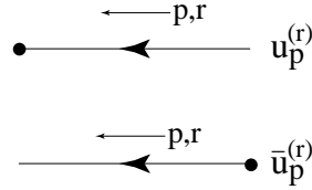
FIG. X.3 Feynman rules for external fermion legs.
