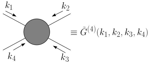
FIG. VIII.3 The blob represents the sum of all Feynman diagrams; the momenta flowing through the external lines is unrestricted.
