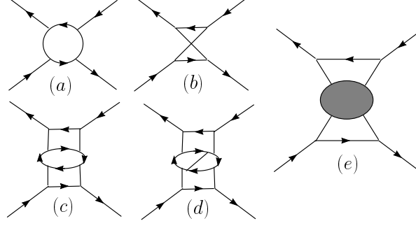
FIG. VIII.4 The graphs in (a-d) all have the form of (e).
