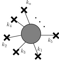
FIG. VIII.7 n 'th order contribution to \langle 0|S|0\rangle in the presence of a source.
