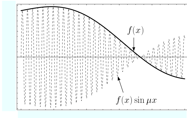
FIG. VIII.8 The Riemann-Lebesgue lemma: f(x) multiplied by a rapidly oscillating function integrates to zero in the limit that the frequency of oscillation becomes infinite.
