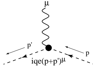
FIG. XI.5 Feynman rule for the derivately coupled charged scalar.
