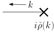
FIG. VIII.6 Feynman rule for a source term \rho(x) .
