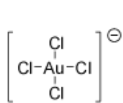
Square planar \text{AuCl}_4^-
