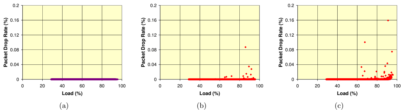
Figure 2: Packet drop rate as a function of load for different buffer sizes. (a) For a buffer size of 190ms we observe no packet drops. Although not shown here, there are also no drops with either 10ms or 5ms of buffering. (b) For a buffer size of 2.5ms packet drops occur in only a handful of cases. (c) When the buffer size is set to 1ms we observe packet drops during high utilization time periods.
