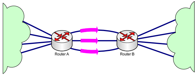
Figure 1: Setup used for buffer sizing experiments in Level 3 Communications' backbone network. The incoming traffic to Router A is divided amongst the three links connecting Router A to Router B using a static hash function to balance the flows.
