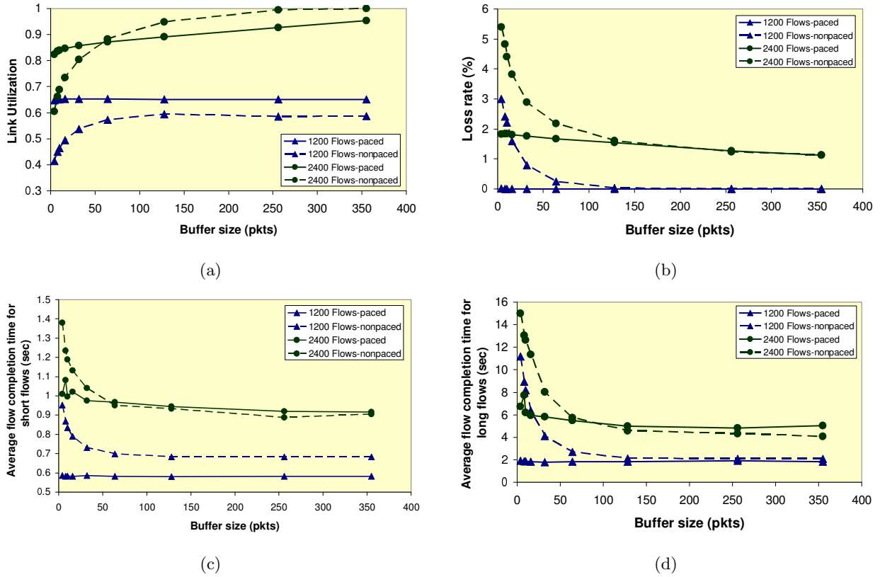
Figure 5: (a) Link utilization as a function of buffer size for paced and non-paced experiments. (b) Loss rate as a function of buffer size for paced and non-paced experiments. (c) Average flow completion times for short-lived flows. (d) Average flow completion times for long-lived flows.
