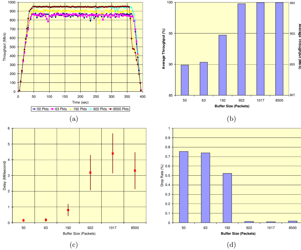
Figure 10: (a) Throughput vs. time for various buffer sizes. (b) Average throughput vs. buffer size. (c) Delay statistics vs. the buffer size. The square represents the average delay and the bar represents the standard deviation. (d) Drop rate vs. buffer size.
