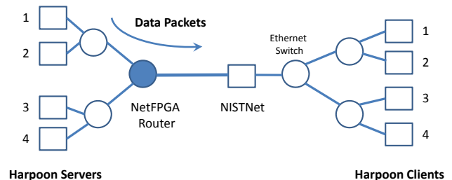
Figure 12: Harpoon Evaluation Topology
