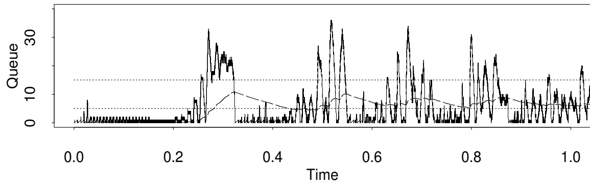
Queue size (solid line) and average queue size (dashed line).
