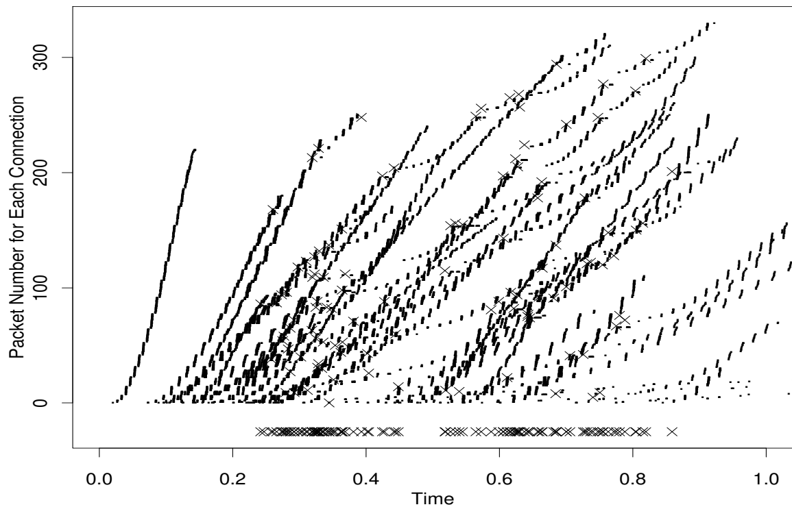
Figure 9: A RED gateway simulation with heavy congestion, two-way traffic, and many short FTP and TELNET connections.
