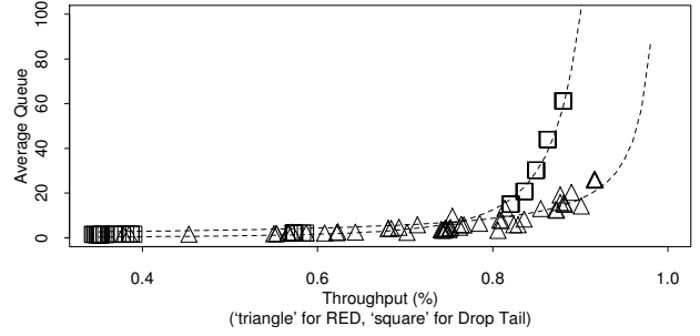
Figure 5: Comparing Drop Tail and RED gateways.
