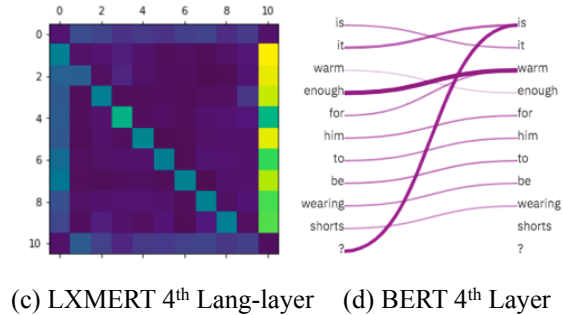
Figure 3: Attention graphs reveal similar behavior in the LXMERT language encoder (a, c) and in the original BERT encoder (b, d). Fig. a & b show the attention pointing to next words while Fig. c & d show the attention pointing to previous words.
