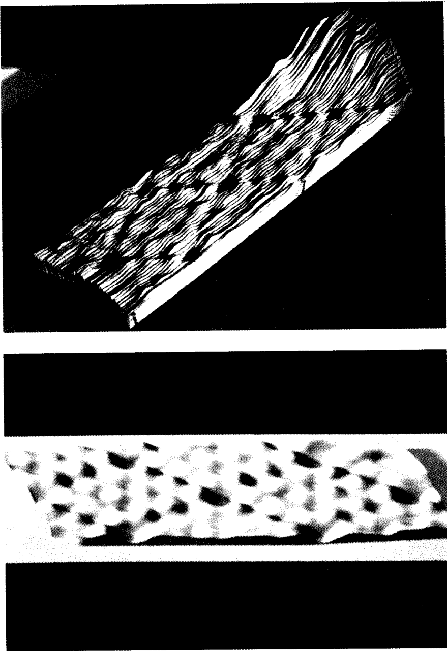
Fig. 6. 7 \times 7 reconstruction of Si(111), (a) Relief assembled from the original recorder traces, from Ref. [19], © 1983 The American Physical Society, and (h) processed image of the 7 \times 7 reconstruction of Si(111). Characteristic of the rhombohedral surface unit cell are the corner hole and the 12 maxima, the adatoms. In the processed image, the six adatoms in the right half of the rhombi appear higher. This is an electronic inequivalence on the surface owing to a structural left-right inequivalence in the underlying layers. The reconstruction extends undisturbed to the immediate vicinity of the large “atom hill” on the right.
